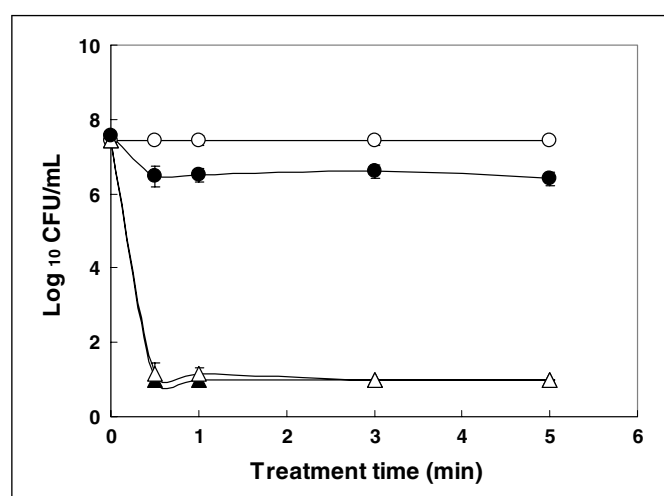
Figure 3 – Reduction of Escherichia coli O157:H7 by sanitizers prepared from flume water. ○, flume water; ●, ClO 2 9 ppm; △, liquid FIT pH 3.0; ▲, dry FIT pH 3.0.
